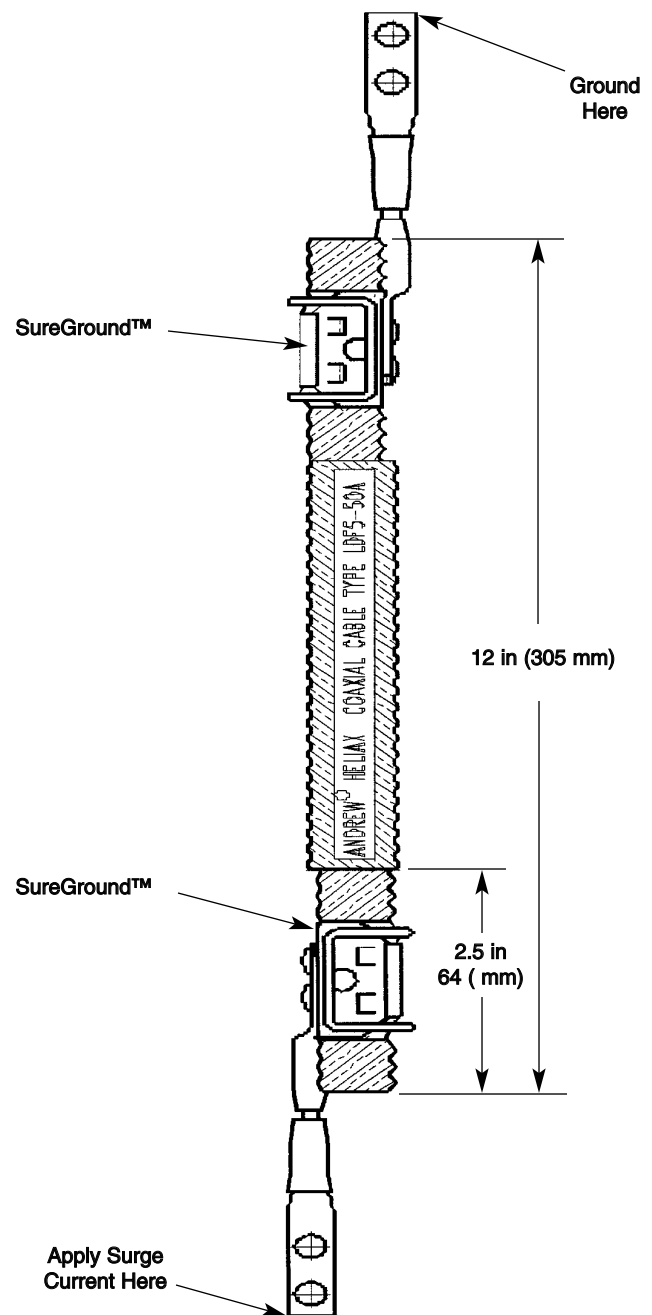
Figure 2 - Setup for Lightning Surge Testing
